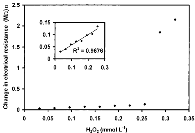
Figure 5 Resistance change behavior of PBMA/PANI-Cl composite film obtained by method I on dipping in H 2 O 2 aqueous solution.
