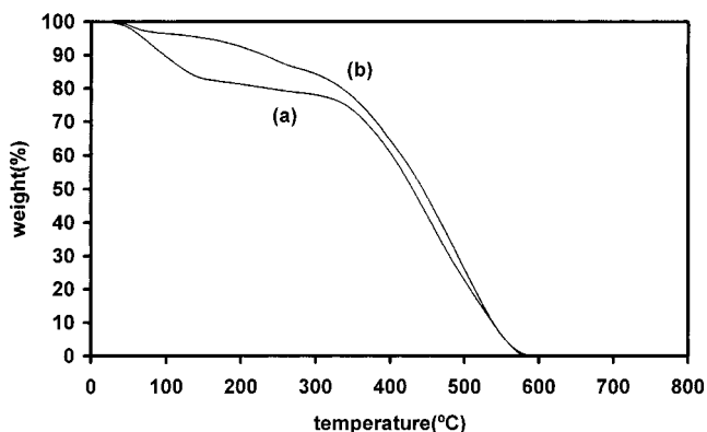
Figure 1 TGA of conducting polymers (a) PANI-Cl and (b) PANI-DBSA.
