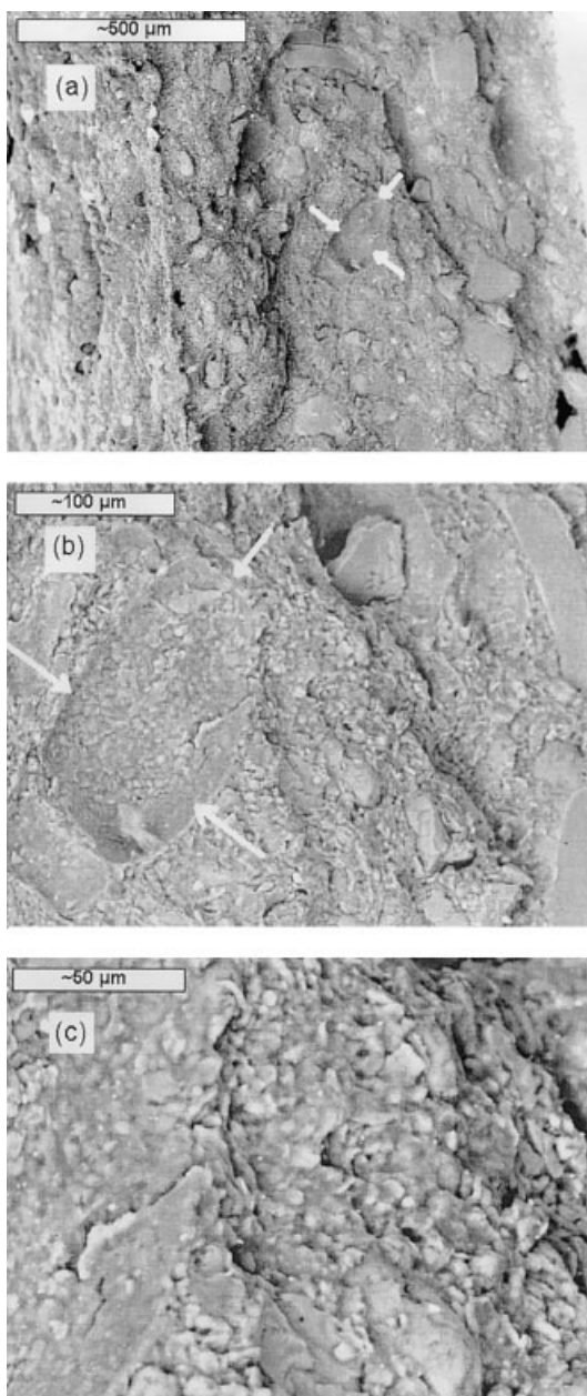
Figure 4 SEM micrographs of composite PBMA (30%)/PANI-DBSA (70%) prepared by method II at different magnifications: (a) 100 \times , (b) 350 \times , and (c) 750 \times .
