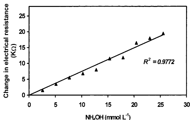
Figure 7 Resistance change behavior of PBMA (30%)/PANI-DBSA (70%) composite film prepared by method II on dipping in \text{NH}_3 aqueous solution.
