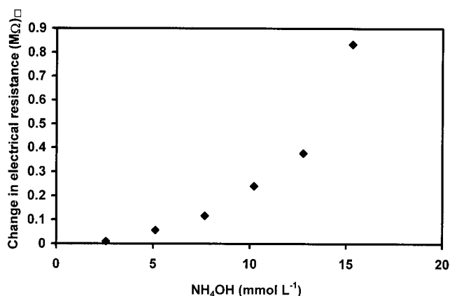
Figure 6 Resistance change behavior of PBMA/PANI-Cl composite film obtained by method I on dipping in NH 3 aqueous solution.
